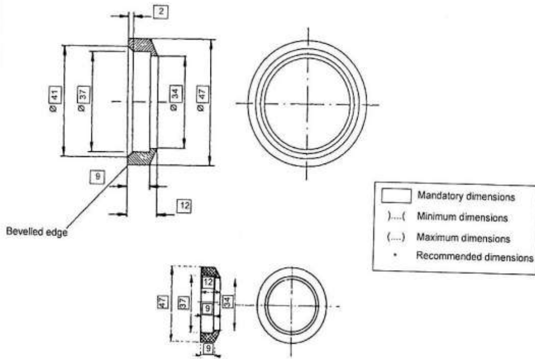
Fig. 34 - Washer
