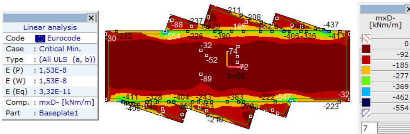
[[], > Baseplate, Linear,(Auto) Critical Min., mxD-, Isosurfaces 2D, Top view
