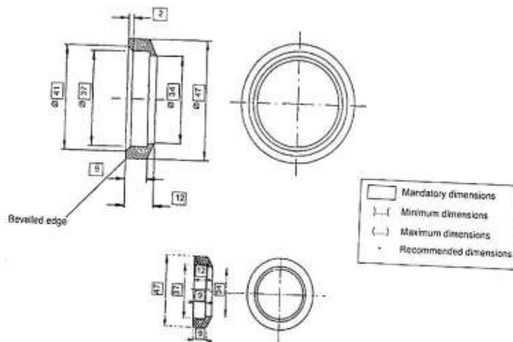
Fig. 34 - Washer
